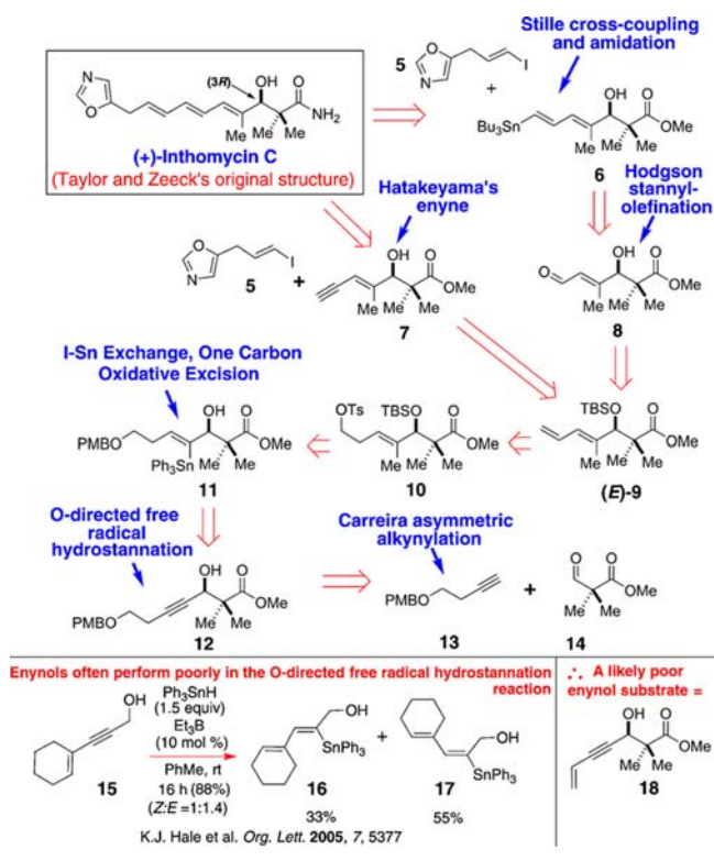
Scheme 2. Our Retrosynthetic Planning for (3R)-(+)-Inthomycin C
