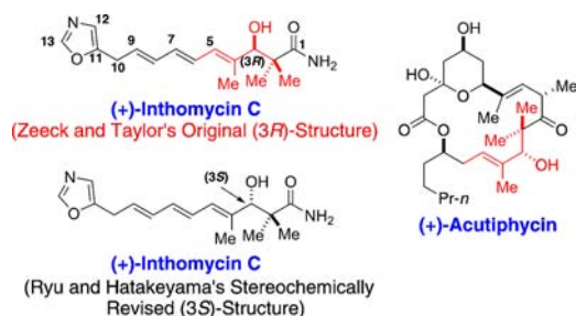
Figure 1. (+)-Inthomycin C and (+)-acutiphycin.
