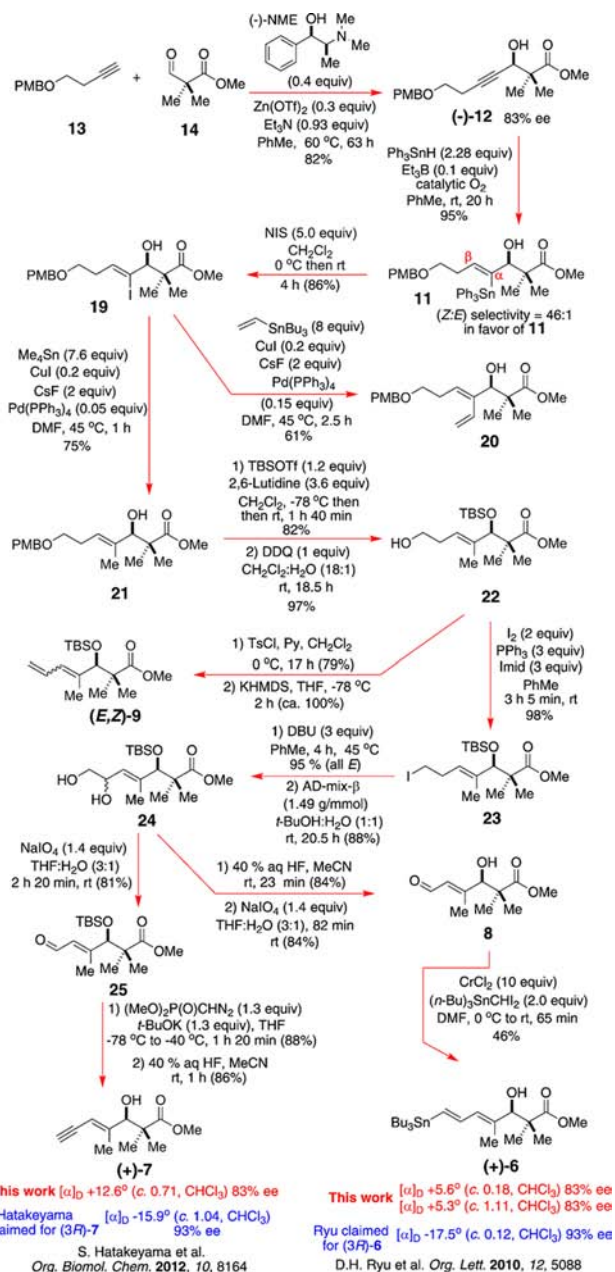
Scheme 3. Our Formal Synthesis of (+)-Inthomycin C that Intersects with Ryu's Claimed Dienylstannane 6 and the Claimed Enyne 7 of Hatakeyama
