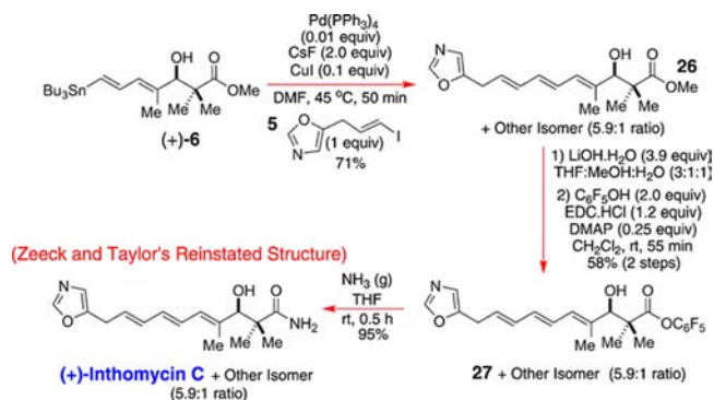
Scheme 4. Our Reinvestigation of the Ryu Cross-coupling of 5 with (+)-6 and Our New Simplified Endgame for Securing the Total Synthesis of (+)-Inthomycin C
