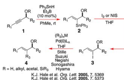
Scheme 1. The O-Directed Free Radical Hydrostannation Route to Trisubstituted Alkenes with Three C–C \sigma -Bonds
